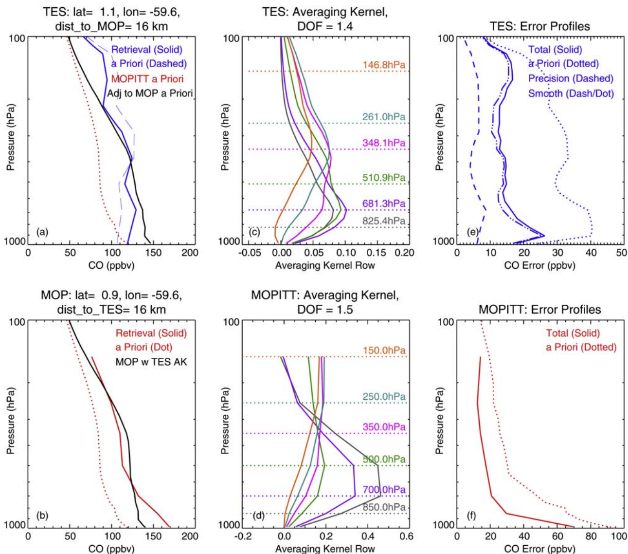
Figure 10. Comparisons of TES and MOPITT retrieved CO profiles in north Brazil, 20 September 2004. (a) TES retrieved CO profile (solid blue curve) and the associated a priori profile (dashed blue curve), the MOPITT a priori (red dotted curve), and the TES retrieval adjusted to the MOPITT a priori (solid black curve). (b) MOPITT retrieved CO profile (solid red curve) and the associated a priori (red dotted curve), and the MOPITT retrieval with TES averaging kernel applied (solid black curve). (c and d) The averaging kernel at six pressure levels from the two instruments. The Degree of Freedom for signal (DOF) is 1.4 and 1.5 for TES and MOPITT. (e and f) Retrieval error breakdown for the two instruments.
