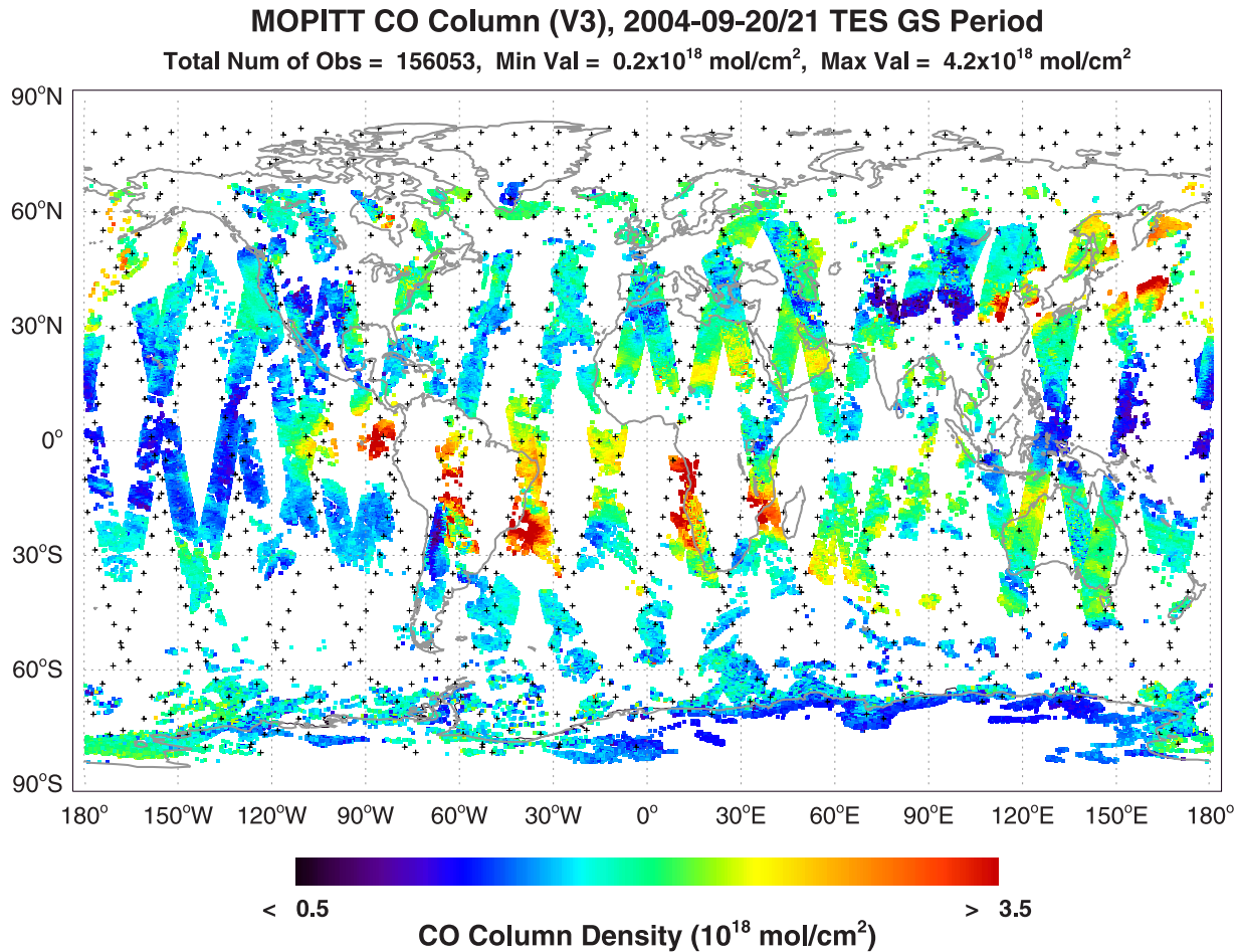
Figure 2. CO total columns from Measurements of Pollution in the Troposphere (MOPITT) measurements during the period of a TES global survey of 20–21 September 2004 (data version 3). Similar to the global CO columns of TES in Figure 1, the MOPITT CO field shows enhanced CO in regions of biomass burning and high-pollution sources. Overlaid black cross symbols are the TES geolocations.
