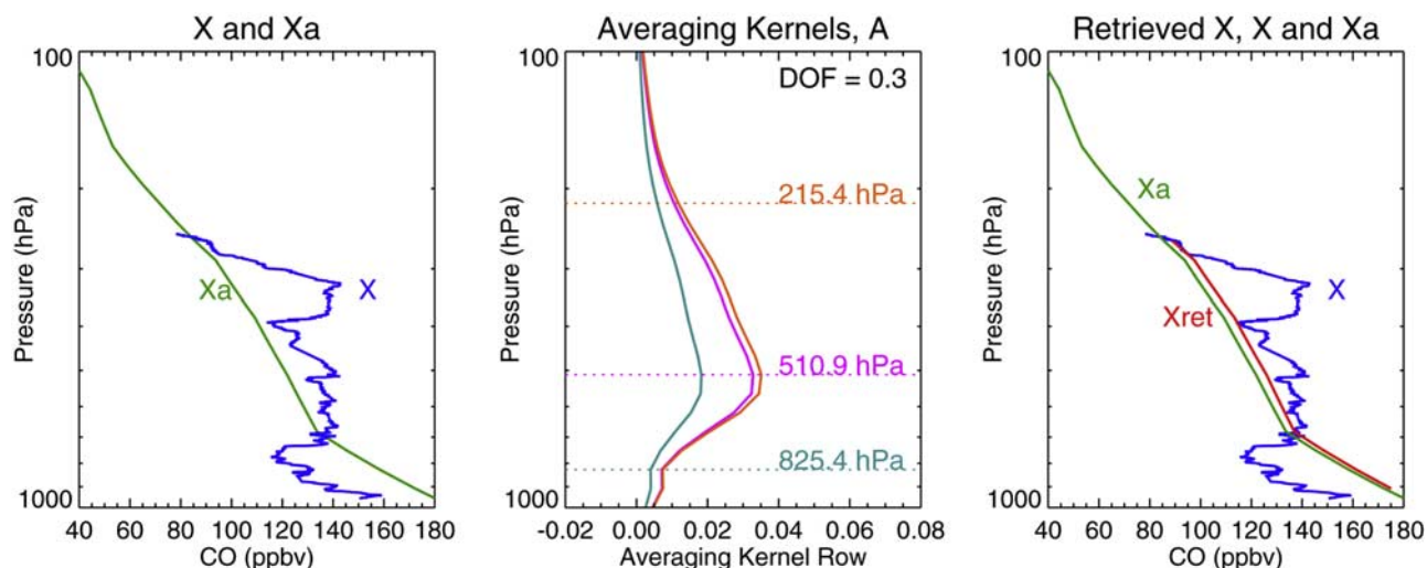
Figure 4. A simulation illustrating the relationship among true, a priori, and the retrieved CO profiles. All three panels are similar to Figure 3. The true CO profile is from the in situ measurement of CO by the DACOM instrument during the Polar Aura Validation Experiment near Portsmouth, 3 February 2005. In this case, the TES retrieval in a close location has DOF of 0.3.
