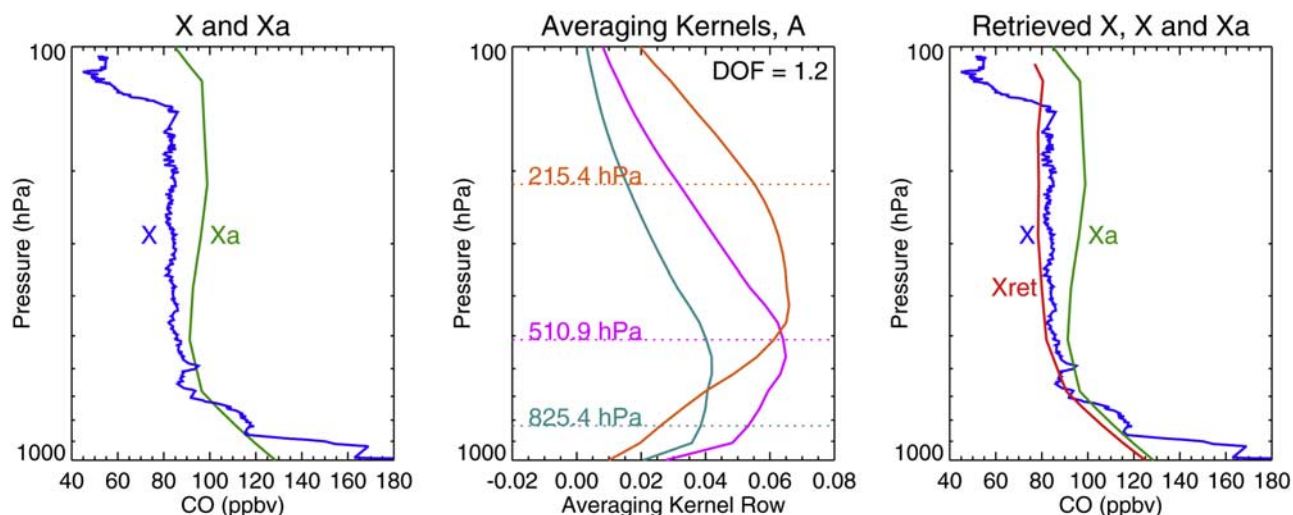
Figure 3. A simulation illustrating the relationship among true, a priori, and the retrieved CO profiles. (left) True CO profile (blue) obtained from in situ measurements of CO from the Argus instrument during Aura Validation Experiment near Houston, 31 October 2004, and the a priori profile (green) used by TES in the closest location. (middle) TES averaging kernel rows corresponding to 825, 510, and 215 hPa for the retrieved profile at the location. The DOF for the TES retrieval is 1.2. (right) Calculated retrieved profile for CO ( x_{ret} , red) together with the true ( x ) and the a priori ( x_a ). The number of CO retrieval levels used in the simulation is 25 between 1000 and 100 hPa.
