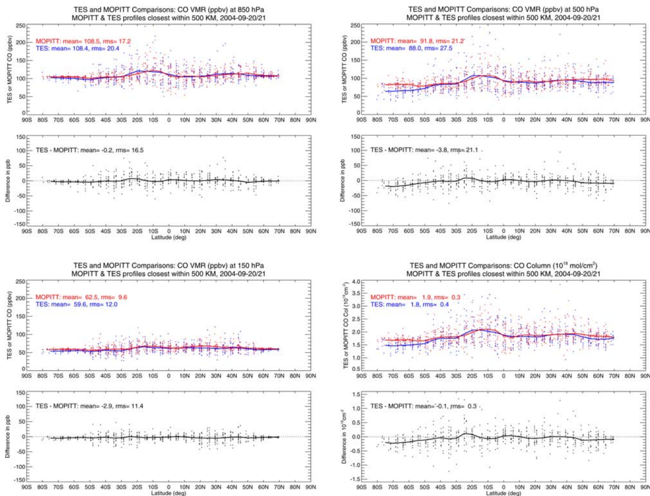
Figure 9. Similar to Figures 7 and 8, this figure shows the comparison between TES and MOPITT CO VMR at three pressure levels and the total column. TES CO profiles are adjusted to MOPITT a priori profile via equation (2). MOPITT CO profiles are adjusted by applying TES averaging kernels via equation (3).
