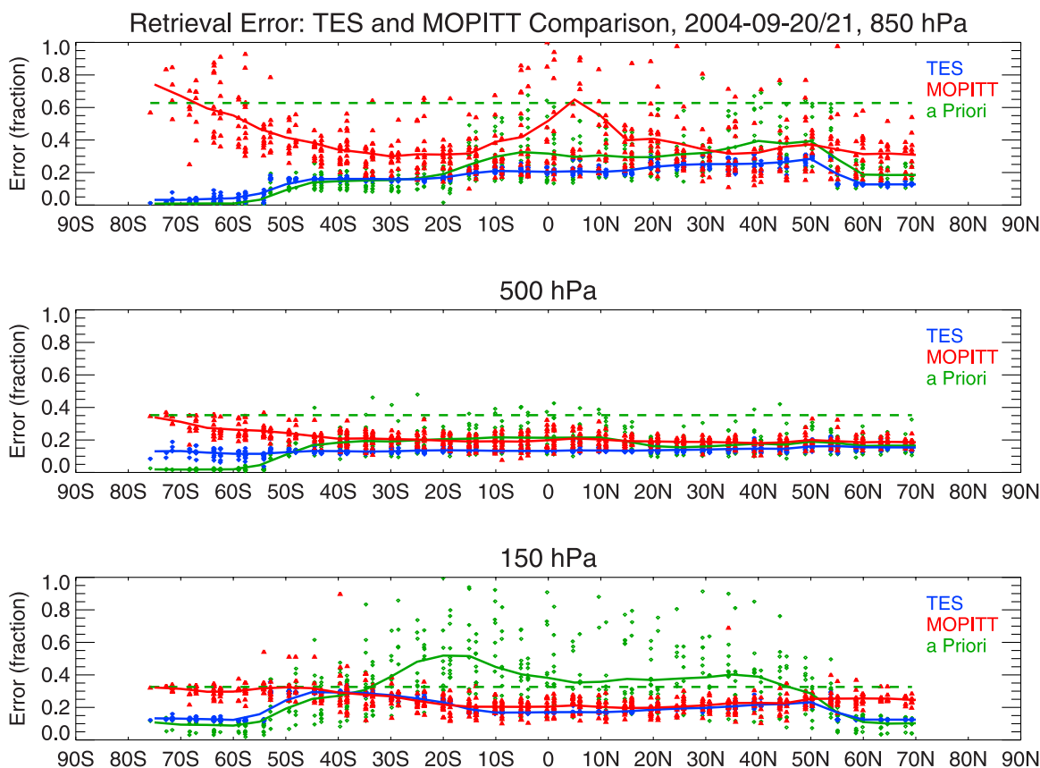
Figure 6. Total CO retrieval errors, as a fraction of the retrieved mixing ratio, reported by TES (blue) and MOPITT (red) and the a priori errors (also as a fraction) (TES = green dots and solid green curve, and MOPITT = dashed green curve) at three pressure levels, 850, 500, and 150 hPa. Solid curves are latitude averages with a bin size of 10^\circ latitude.
