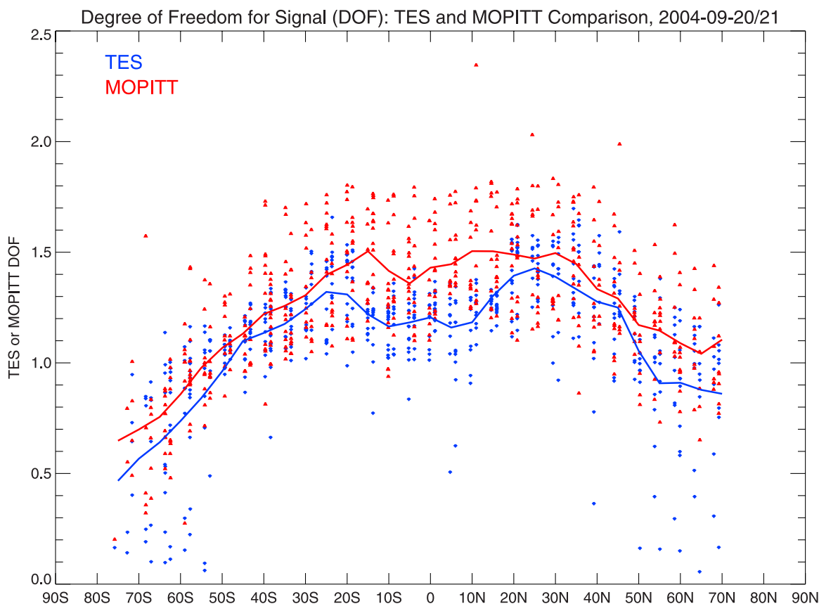
Figure 5. Degrees of Freedom for Signal (DOF) of CO profile retrievals as a function of latitude from TES (blue) and MOPITT (red). MOPITT data are selected for each TES data point at closest location in a TES global survey period of 20–21 September 2004. Latitude averages in a \pm 5^\circ bin are shown in solid curves for the two instruments.
