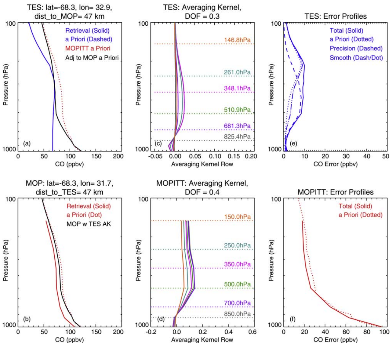
Figure 11. Similar to Figure 10, comparisons of TES and MOPITT retrieved CO profiles over ocean in Southern Hemisphere, 20 September 2004. The Degree of Freedom for signal (DOF) for this case is 0.3 and 0.4 for TES and MOPITT, respectively.
