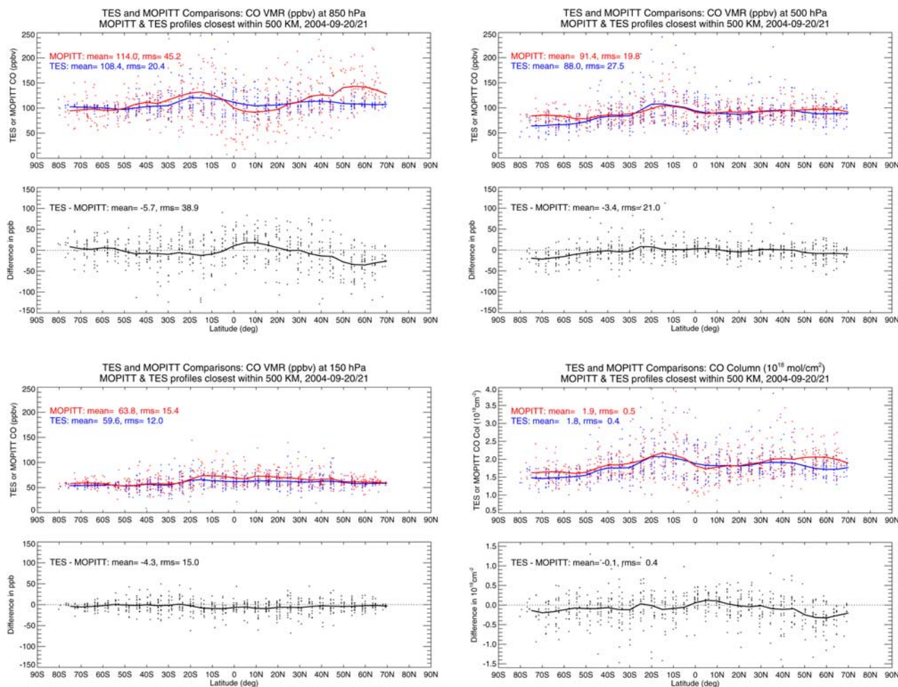
Figure 8. Similar to Figure 7, this figure shows the comparison between TES and MOPITT CO VMR at three pressure levels and the total column. TES CO profiles are adjusted to MOPITT a priori profile via equation (2).
