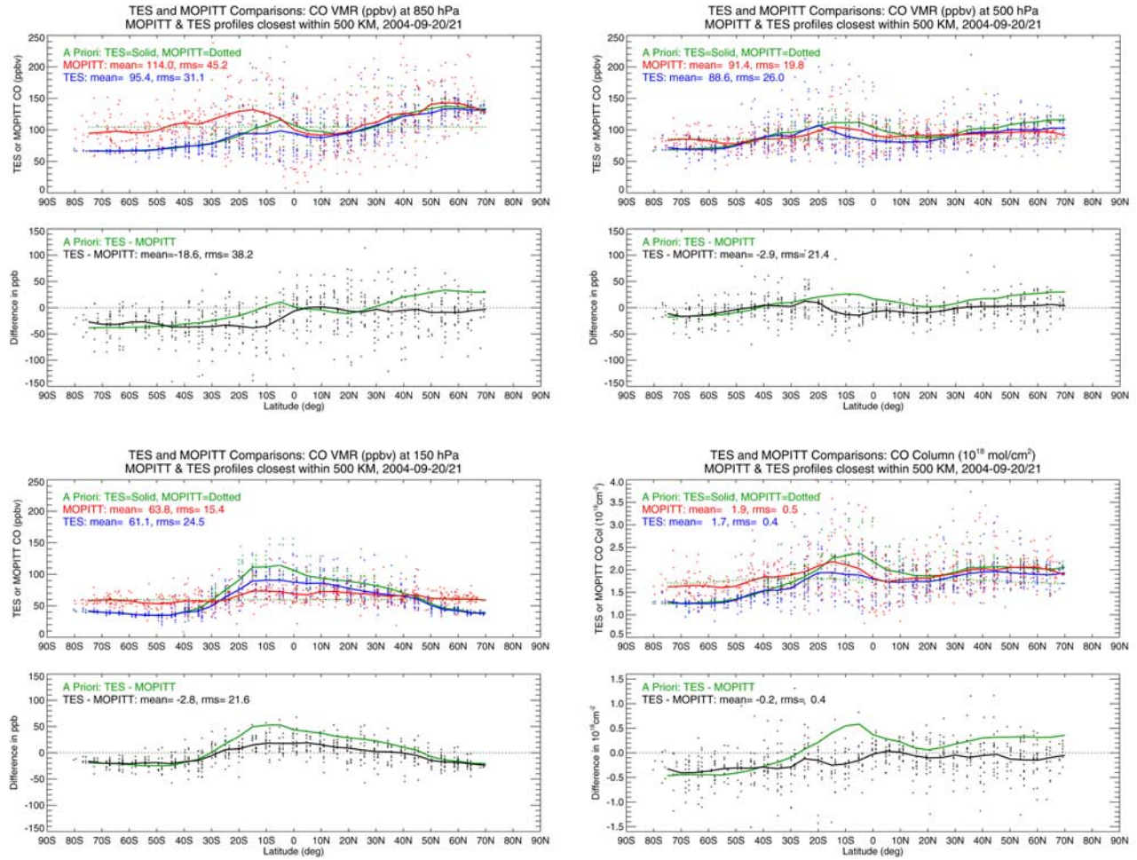
Figure 7. Comparisons of CO Volume Mixing Ratio (VMR) at three pressure levels, 850, 500, and 150 hPa and the total CO column reported by TES and MOPITT. For each pressure level or the total column, there are two panels, the TES and MOPITT data comparison and the difference between TES and MOPITT. In each top panel, TES and MOPITT CO VMR are shown in blue and red, respectively, and the TES and MOPITT a priori are shown in green with TES averages being shown as solid curves and MOPITT single value being shown as a dashed line. In each bottom panel, CO VMRs of TES minus MOPITT are shown in black, and the difference in a priori is shown in green. The global averages (mean) and the root mean squares (rms) of the comparison data are provided.
